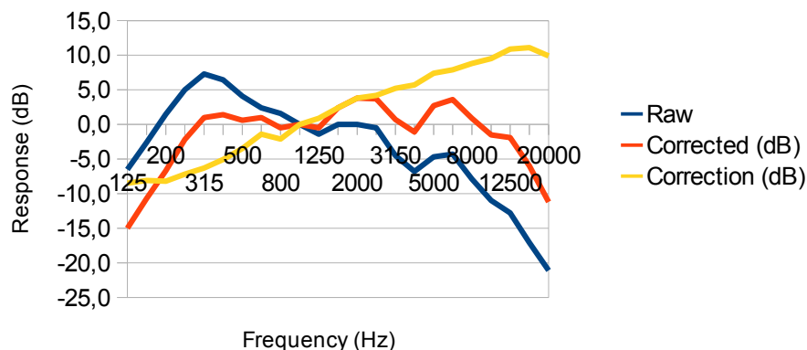
SICP70 frequency response
